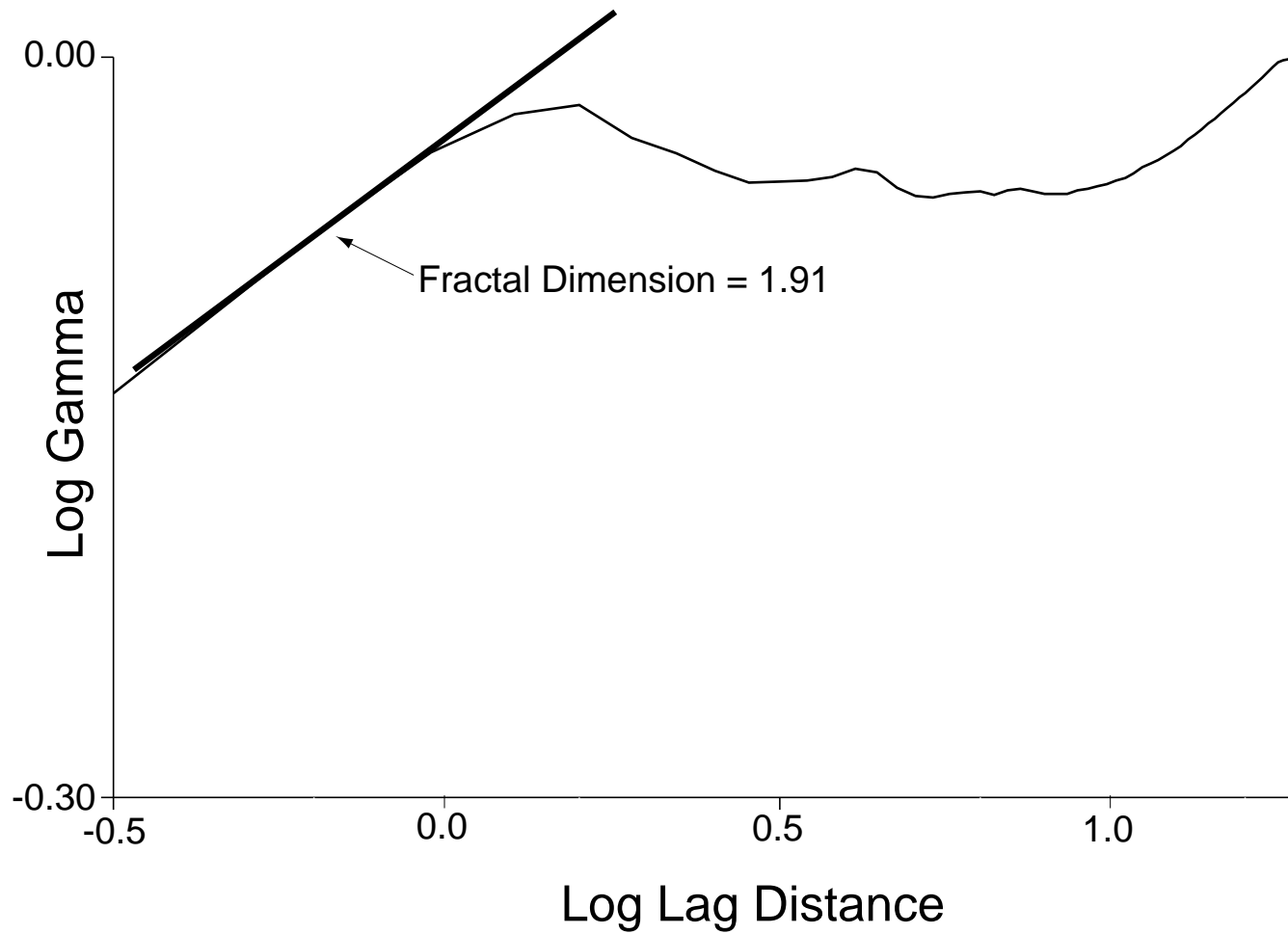
Figure 40 Variogram hydraulic conductivity data from Figure 38 plotted on a log-log plot
